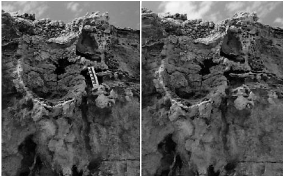
Figure 2: Stereopair of the hemispherical base, with thin cemented rim, of a pipe at 'The Petrified Forest', Victoria, about 30 m west of the main group shown in Figure 1. Scale-bar is 10 cm.
