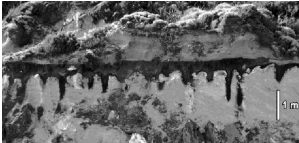
Figure 4: A red paleosol and soil-filled pipes beneath a younger sand dune exposed in a cliff at Canunda National Park, South Australia. These pipes lack a cemented rim.
